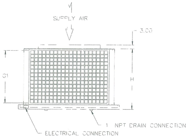
ELEVATION VIEW
